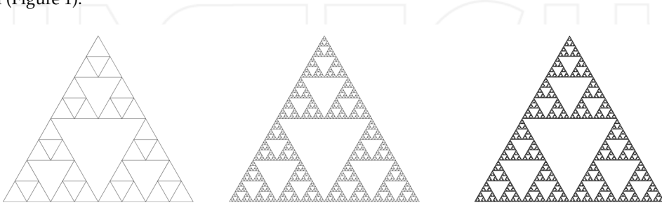
Figure 1. Sierpinski triangle: starting with a simple initial configuration of units or with a geometrical object then the simple seed configuration is repeatedly added to itself in such way that the seed configuration is regarded as a unit and in the new structure these units are arranged with respect to each other according to the same symmetry as the original units in the seed configuration. And so on.
